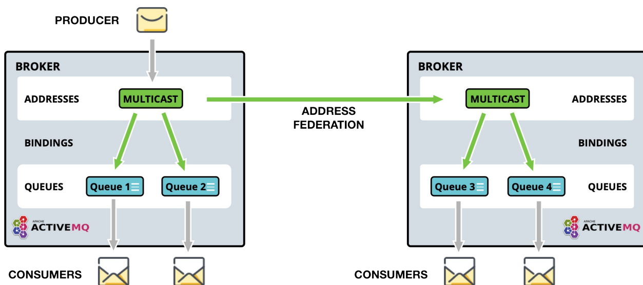
Figure 1. Address Federation
