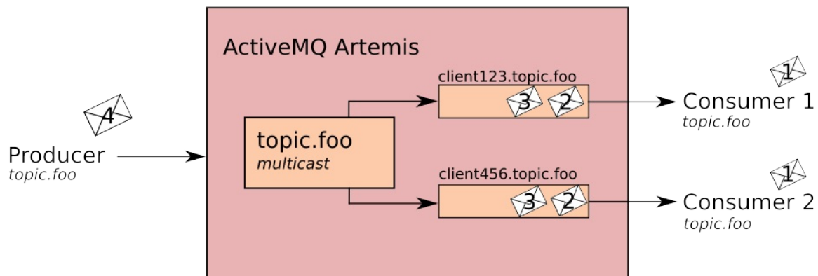
Figure 2. Publish-Subscribe
